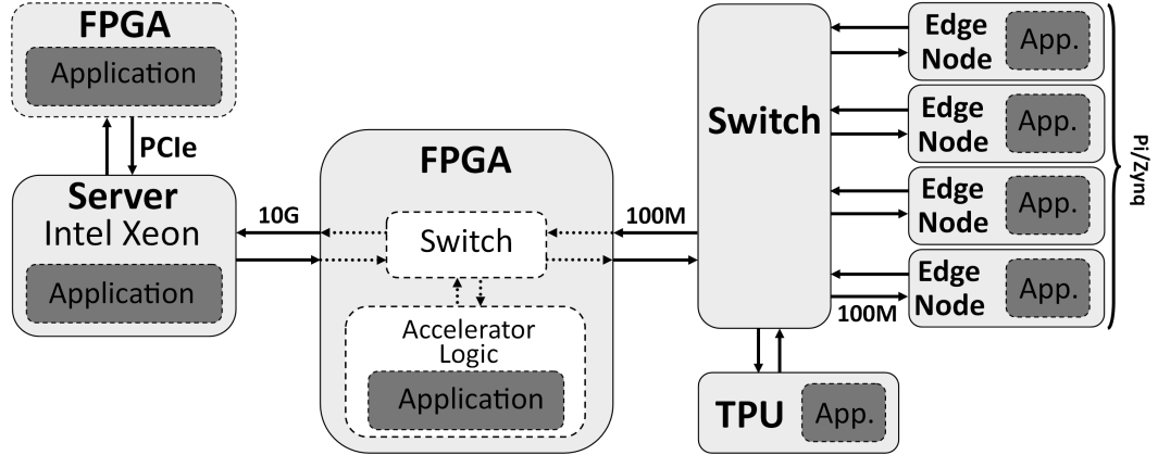
Figure 5.1: Outline of the experimental set up - images are sent from the edge node through the network switch to the Server. In these experiments, latency is measured as the total latency to complete the computation on each platform, returning the result to the source node, including communication time.
