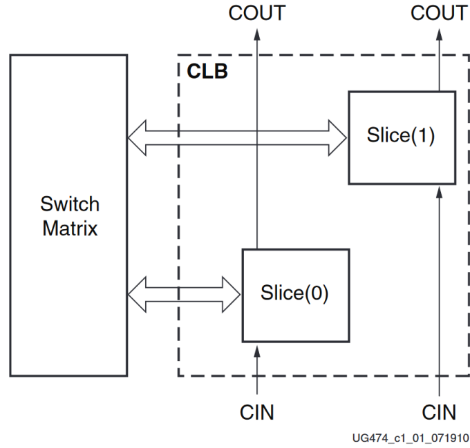
Figure 2.2: Xilinx 7 Series CLB arrangement [24]
