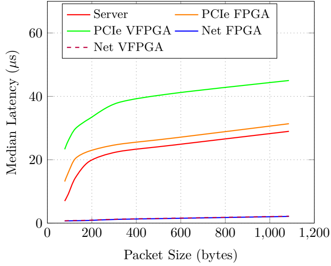
Figure 4.5: Median latency for differing packet sizes.
