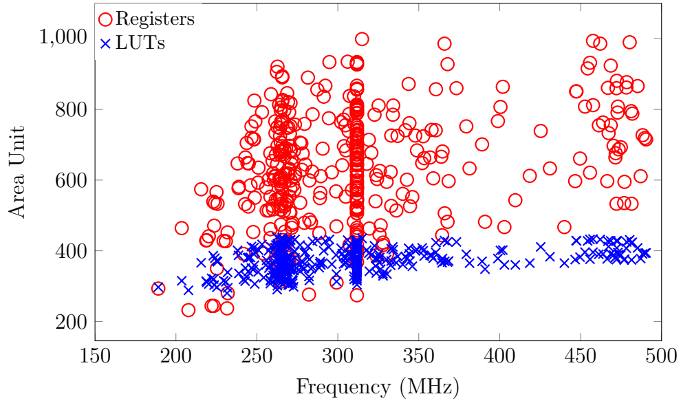
FIGURE 6.9: Resource utilization of all pipeline combinations with internal loopback.
