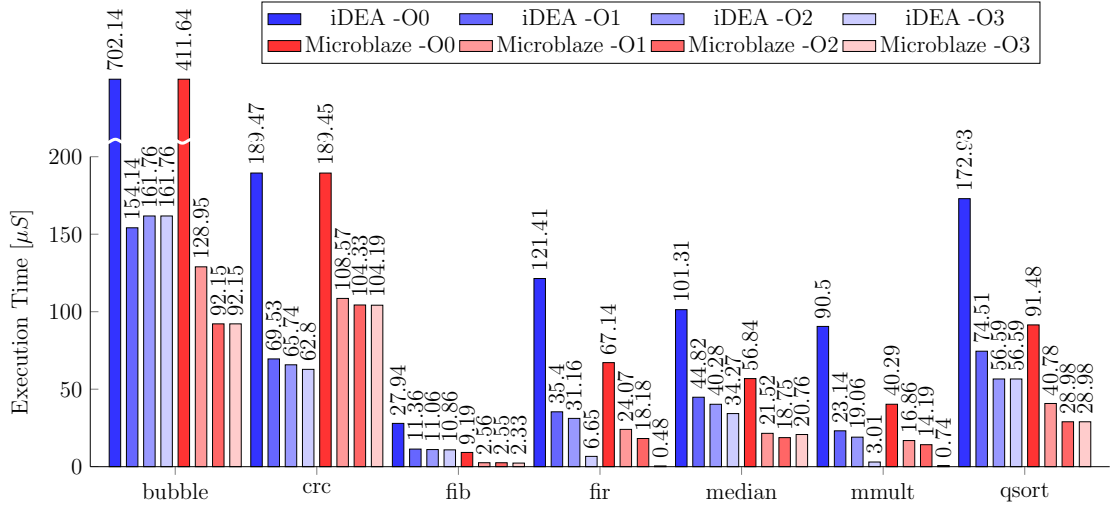
FIGURE 4.6: Comparison of execution time of iDEA and MicroBlaze at maximum pipeline-depth configuration.
