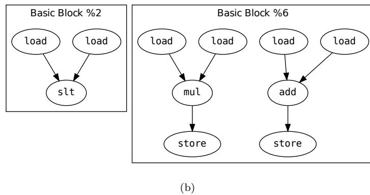
FIGURE 5.3: (a) Control flow graph (b) Dependence graph for a multiply-add function.
