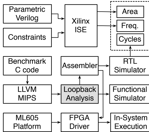
FIGURE 6.7: Experimental flow.
