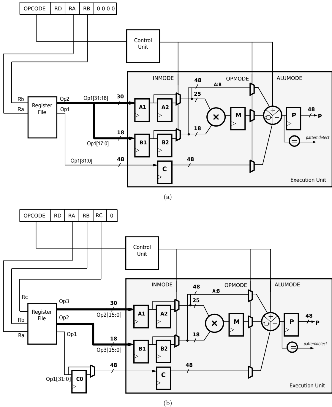
FIGURE 4.3: (a) 2-operand (b) 3-operand input map.
