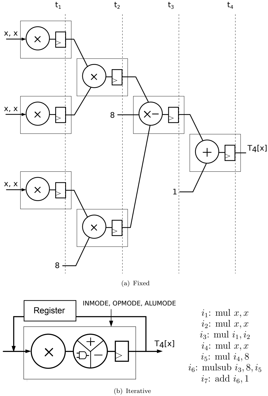
FIGURE 3.9: Implementing Chebyshev polynomial on FPGA. Polynomial equation: T_4[x] = 8x^4 - 8x^2 + 1
