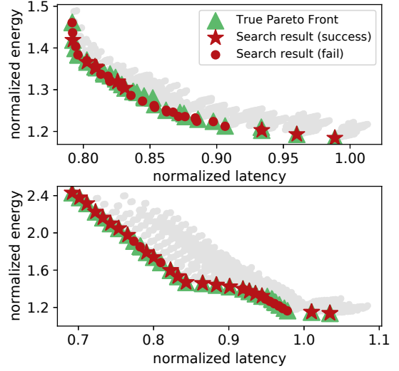
Fig. 12: Experimental results for multiple splits on VGG16 ( \uparrow ) and ResNet50 ( \downarrow ) for CIFAR-100 (batch size=1).
