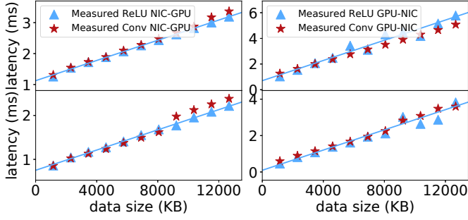
Fig. 10: Comparison of ReLU-based and Conv-based NIC-GPU ( \leftarrow ) and GPU-NIC ( \rightarrow ) latencies on Jetson Orin Nano ( \uparrow ) and AGX Orin ( \downarrow ).
