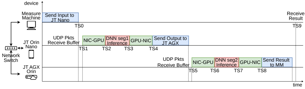
Fig. 3: Illustration of measurement setup showing the measurement machine that initiates measurements and the measured components.
