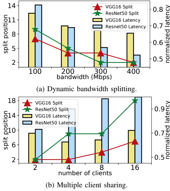
Fig. 13: Experimental results for single split on VGG16 and ResNet50 for CIFAR-100 under dynamic bandwidth and with multiple clients.
