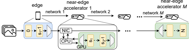
Fig. 1: Split DNN system architecture.
