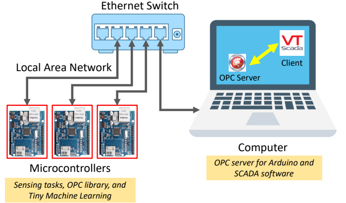
Fig. 2. Scenario of the SCADA/HMI system.
