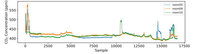
Fig. 1. Concentration of CO 2 in three different rooms.
